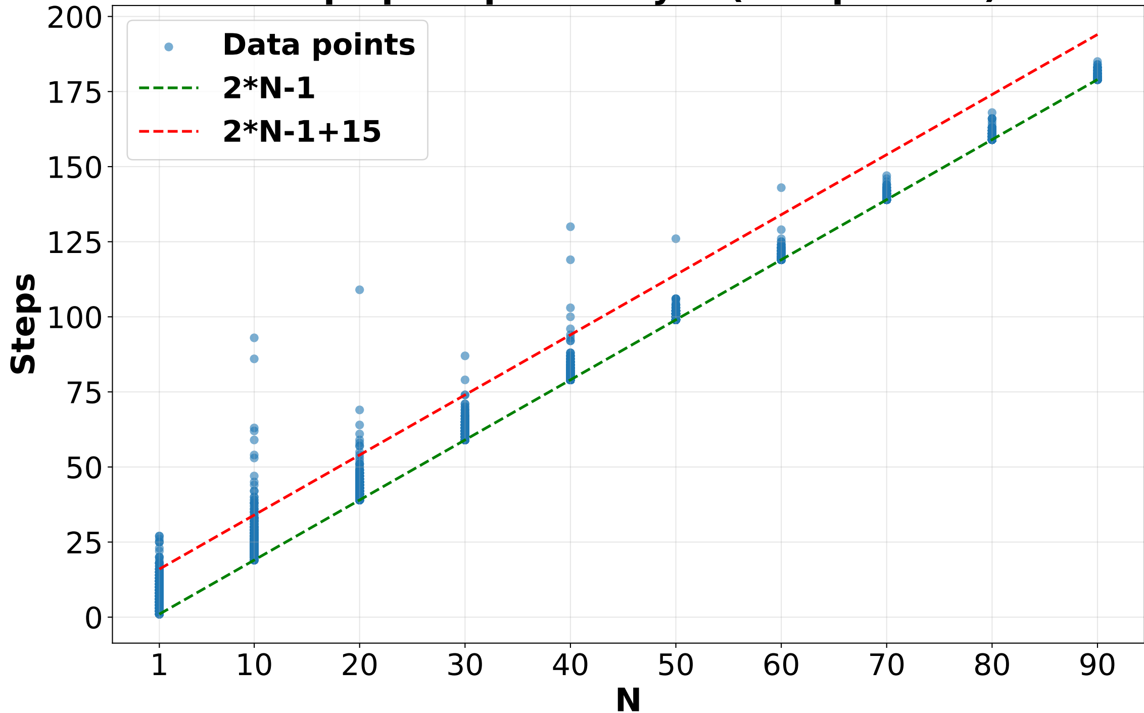
Steps per Episode by N (All Episodes)
