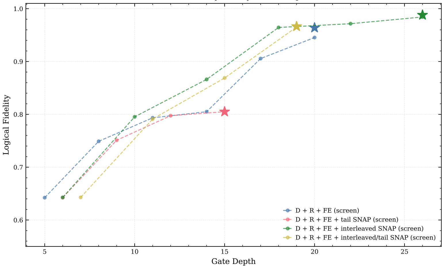
Cluster-Unitary Fidelity vs Gate Depth
