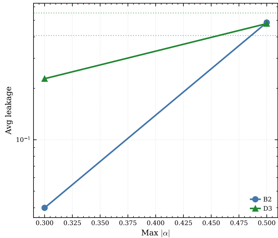
(c) Leakage at N_{cav}=12
