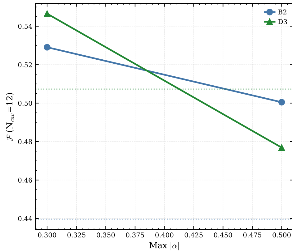
(b) Physical fidelity ( N_{cav}=12 )
