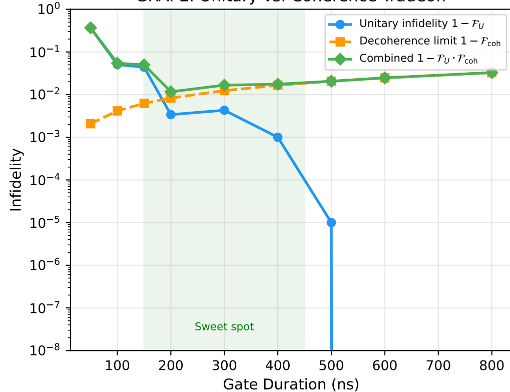
GRAPE: Unitary vs. Coherence Tradeoff
