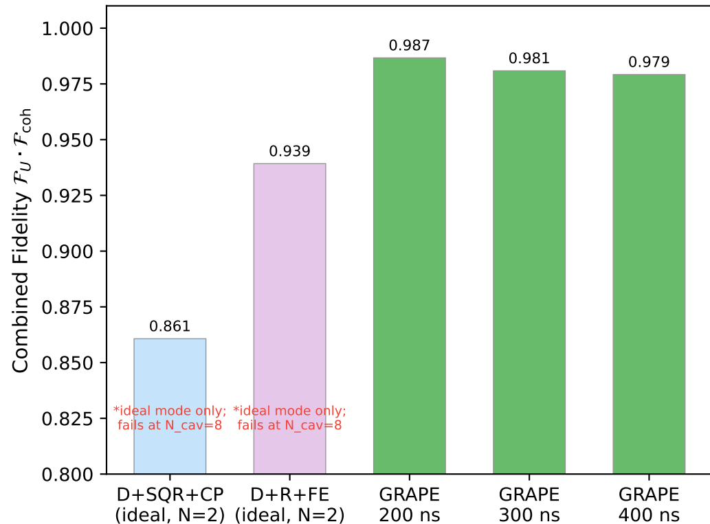
Strategy Comparison with Decoherence
