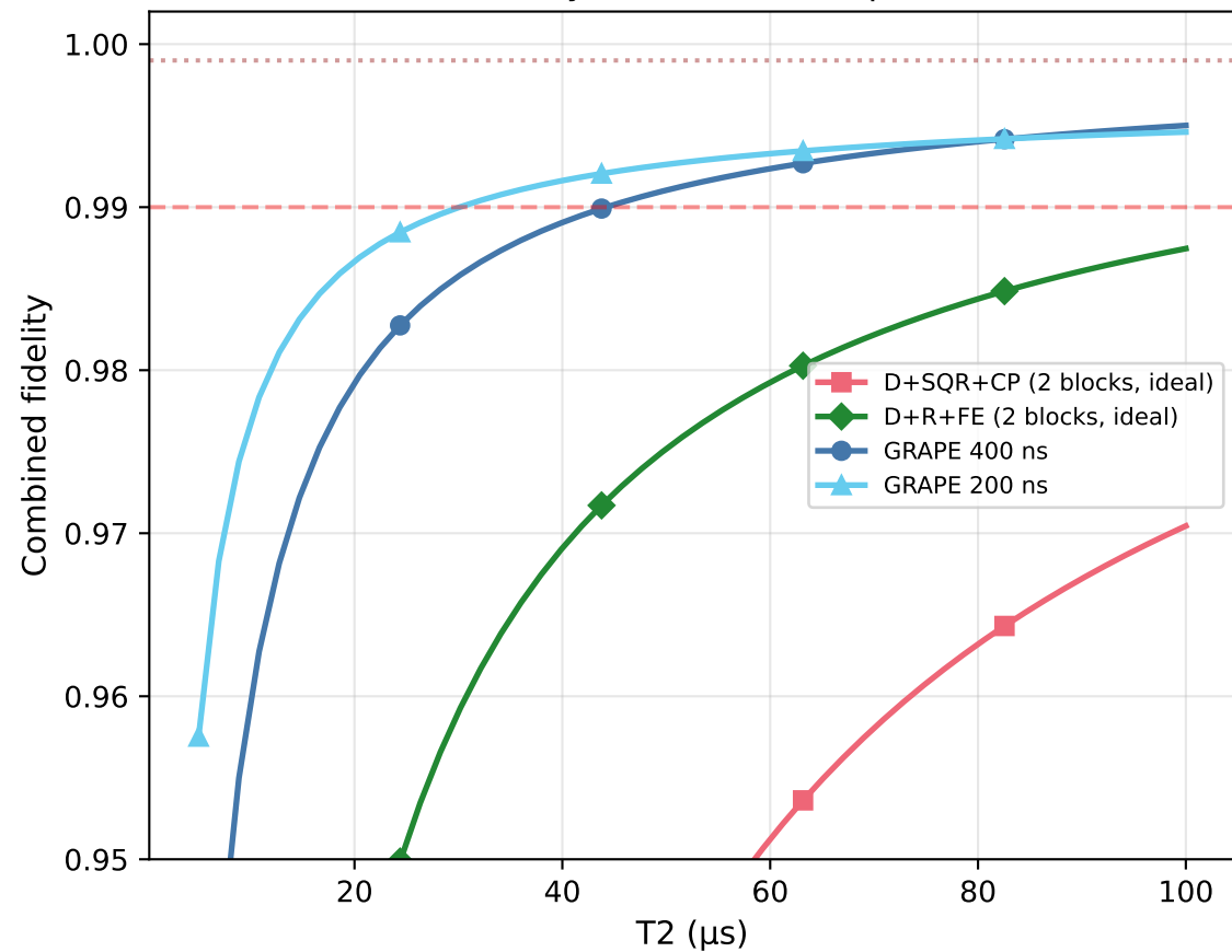
Fidelity vs T2 ( T_1 = 30\ \mu\text{s} )
