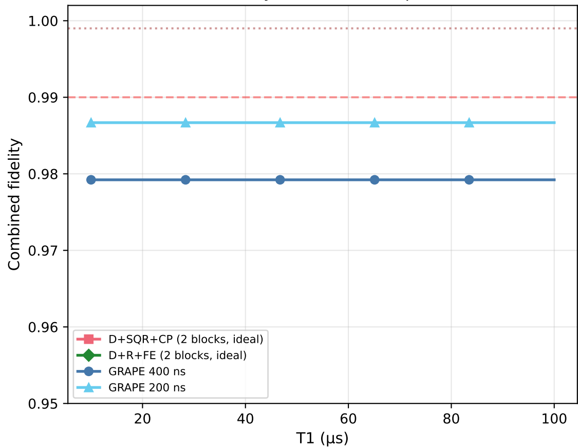
Fidelity vs T1 ( T_2 = 20\ \mu\text{s} )
