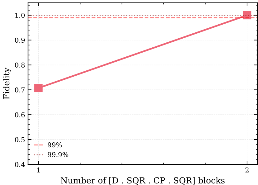
D + SQR + CP: Fidelity vs Depth
