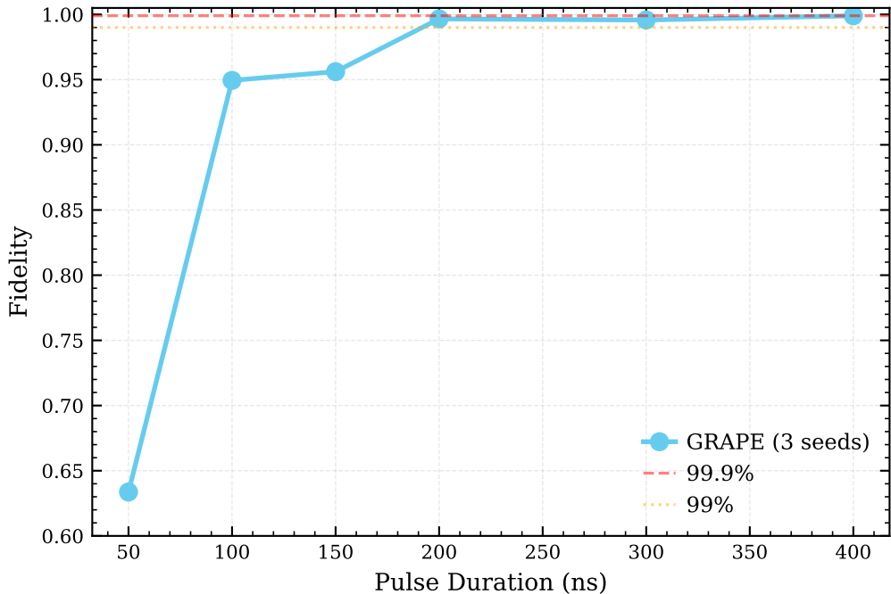
GRAPE Fidelity vs Duration — Cluster-State Target
