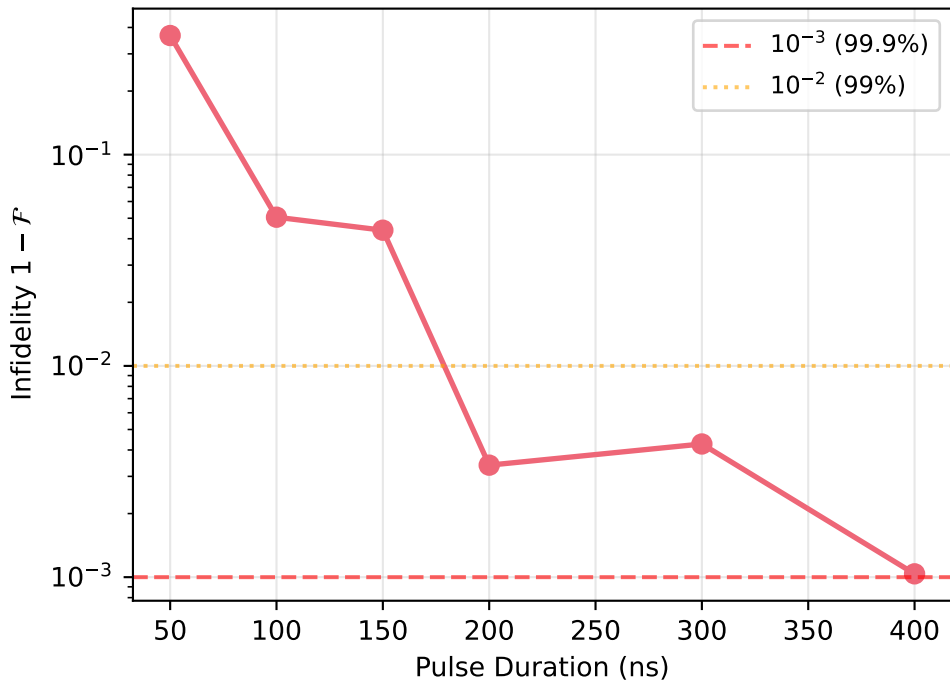
GRAPE Infidelity vs Duration
