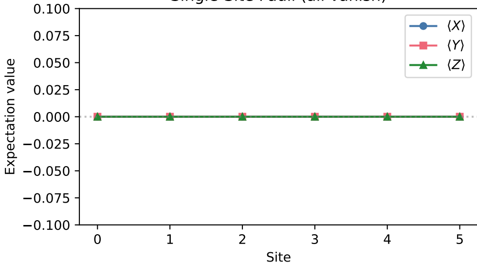
Single-Site Pauli (all vanish)
