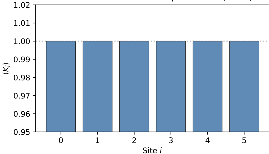
Cluster-State Stabiliser Expectations ( N = 6 )
