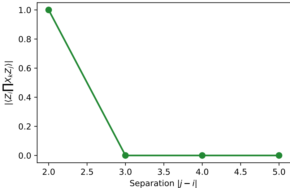
String-Order Correlator vs Separation
