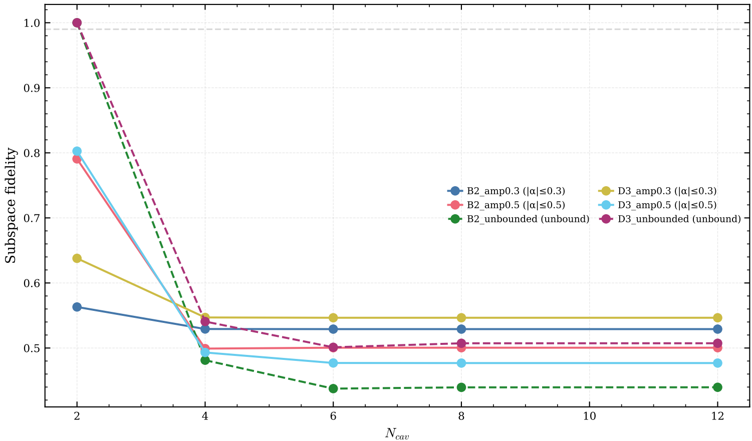
Truncation Convergence: Bounded vs Unbounded
