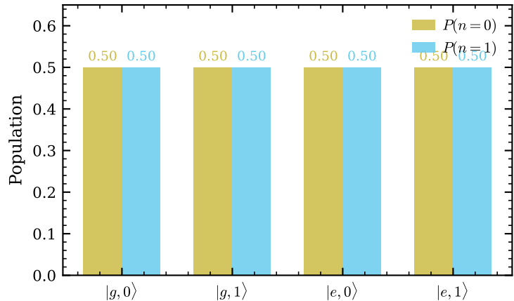
Cavity Fock populations (output of U_{\text{target}} , exact)
