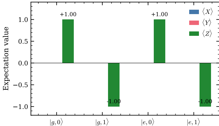
Transmon Bloch-vector components (output of U_{\text{target}} , exact)
