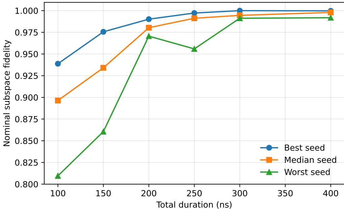
GRAPE Benchmark Frontier
