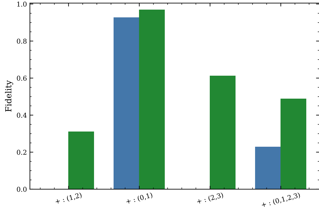
Representative CPSQR primitive: probe-state diagnostics \min(\text{full})=0.0000 , \min(\text{cav})=0.3114
