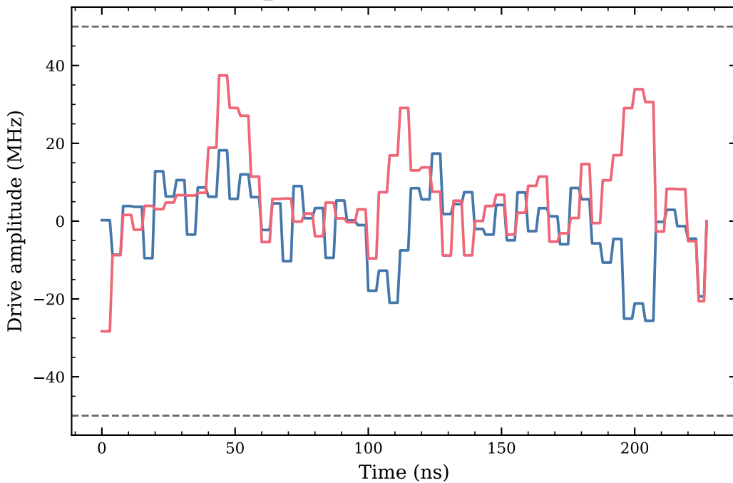
Representative CPSQR primitive: CP2 F_{\text{sub}}=0.4754 , peak=41.6 MHz
