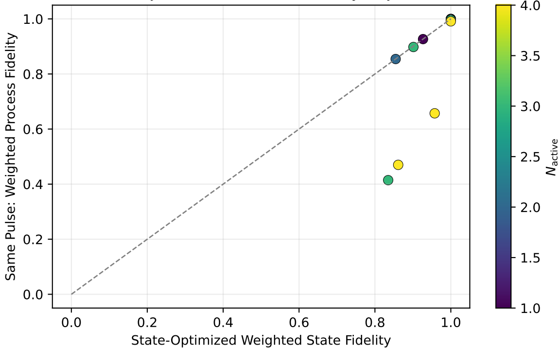
State Objective vs Effective-Unitary Objective
