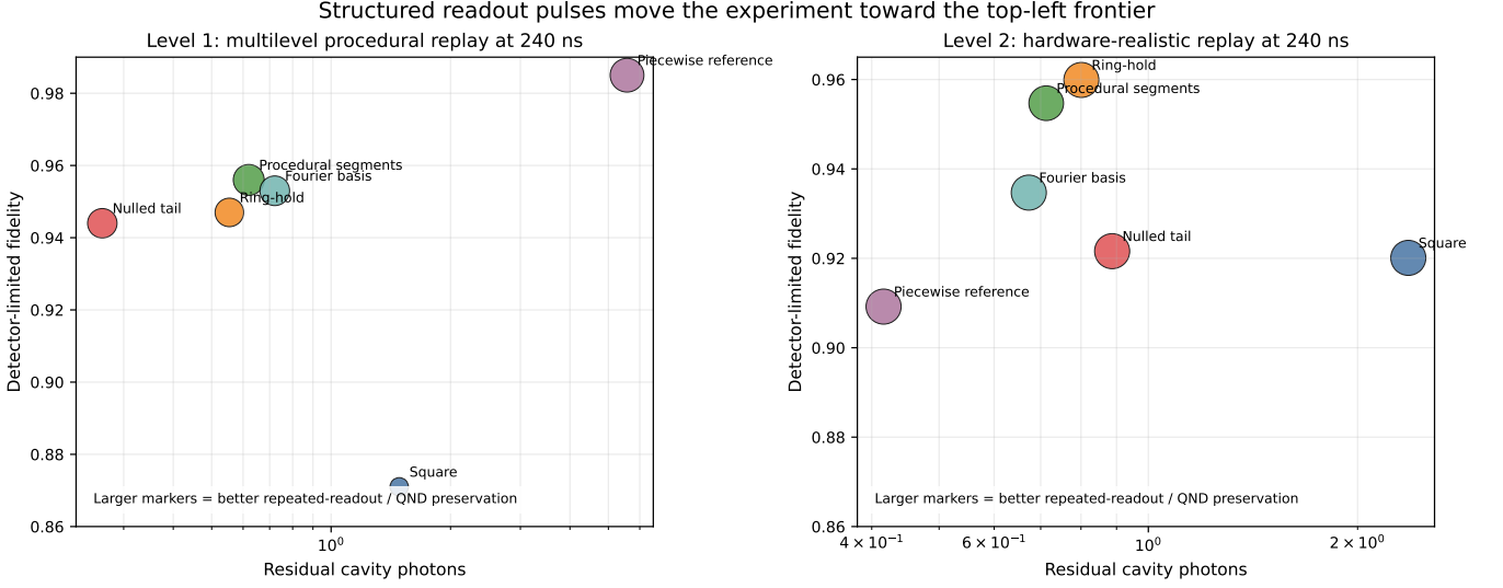
FIG. 1. Experiment-facing frontier at the representative 240 ns operating point. Left: multilevel replay. Right: hardware-realistic replay with QND penalties. In both panels, moving toward the upper-left corresponds to better assignment fidelity with fewer residual photons, and larger markers indicate better repeated-readout preservation. The ring-hold family is the best practical frontier point once hardware transport and QND penalties are included.
