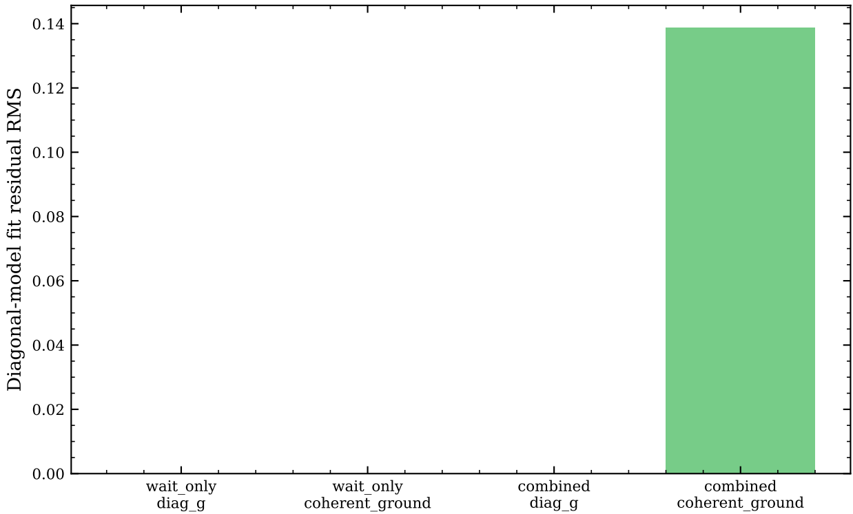
Cavity-Coherence Witness
