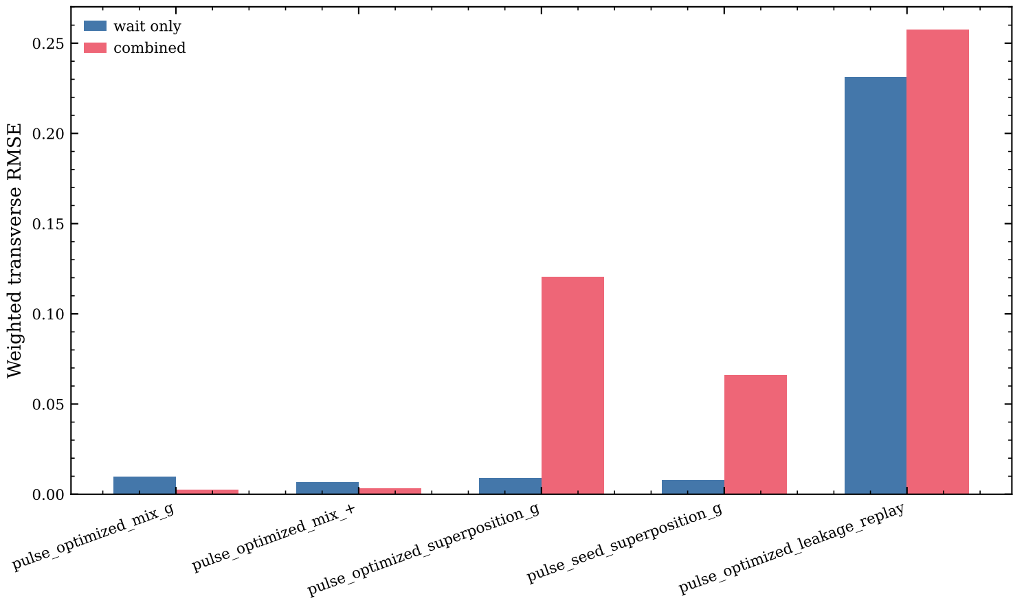
Pulse-Level Black-Box Case Recovery
