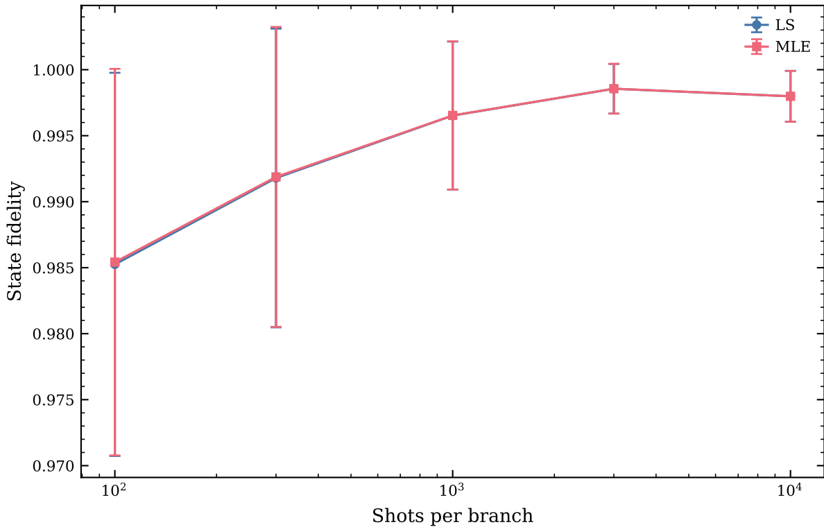
Single-Qubit Tomography Baseline
