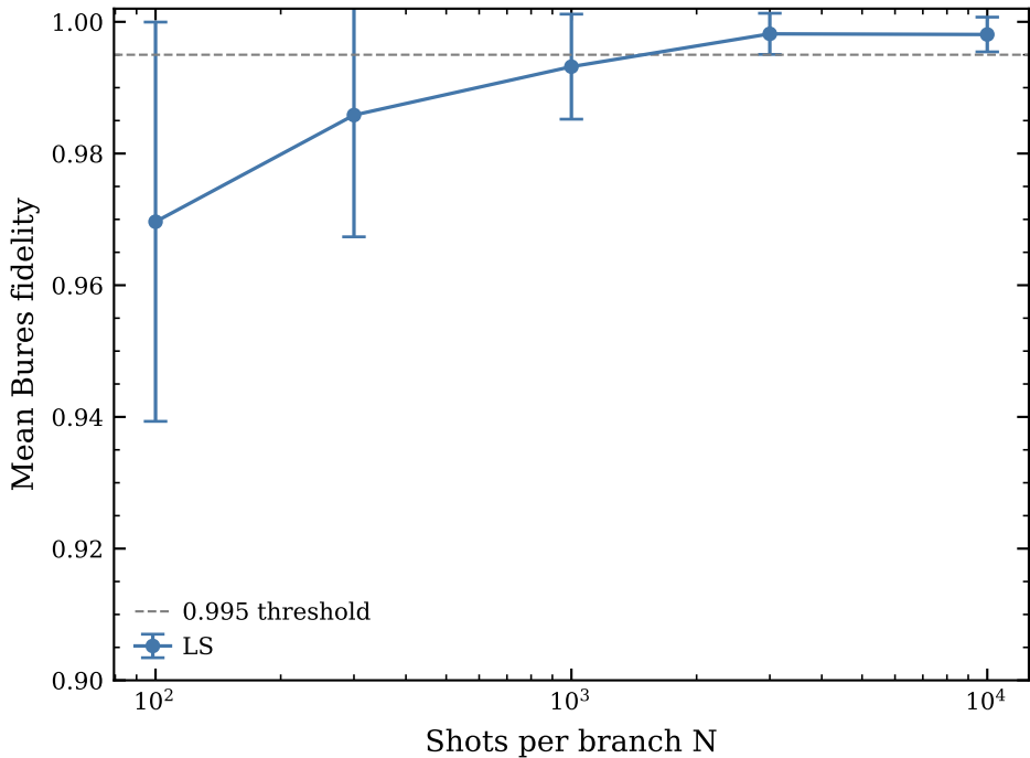
Part 1 single-qubit baseline — LS
