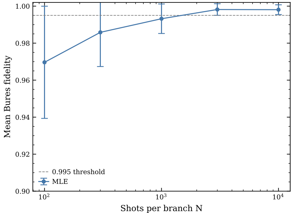
Part 1 single-qubit baseline — MLE
