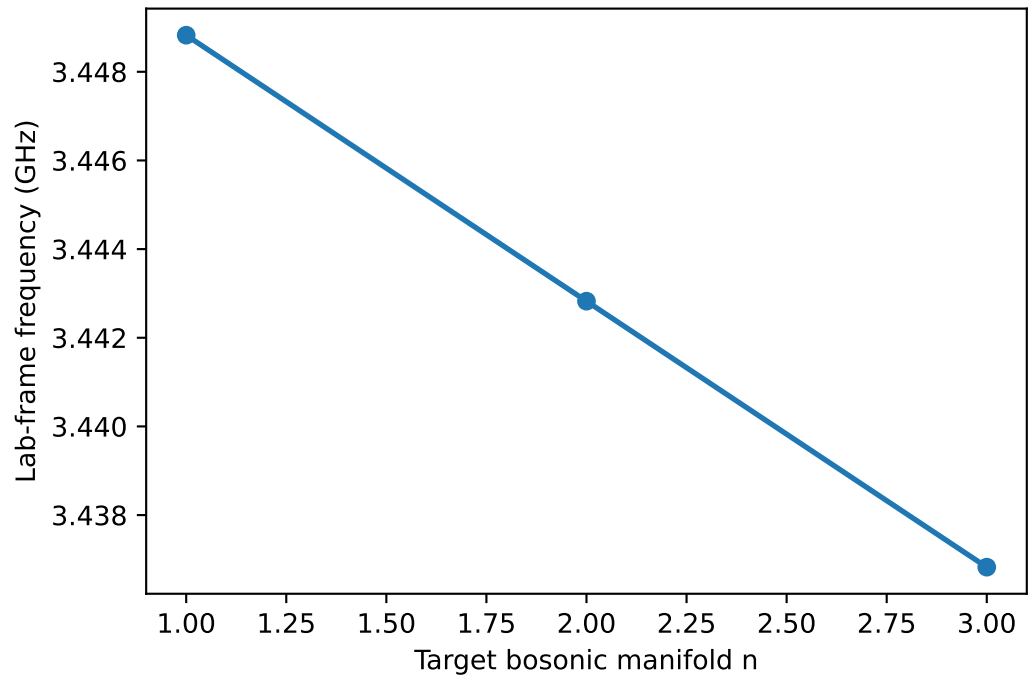
Readout sideband frequency map
