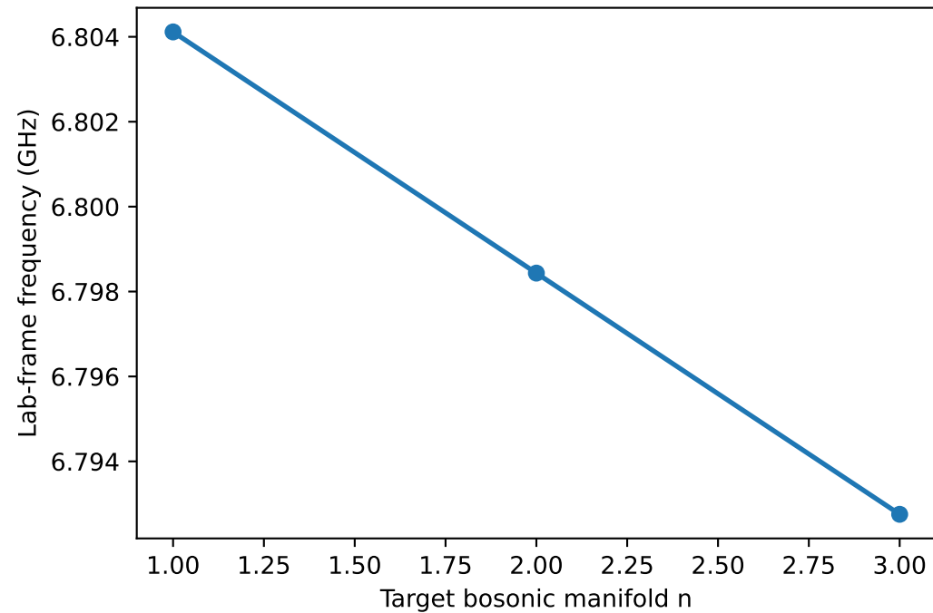
Storage sideband frequency map
