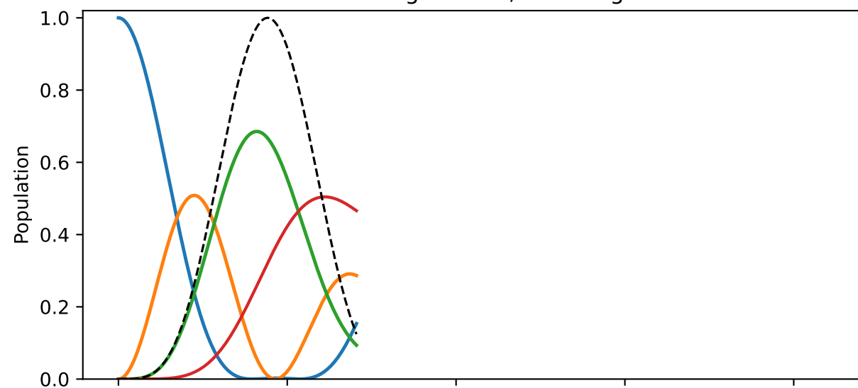
n=3 resonant: g=4 MHz, detuning=0 MHz
