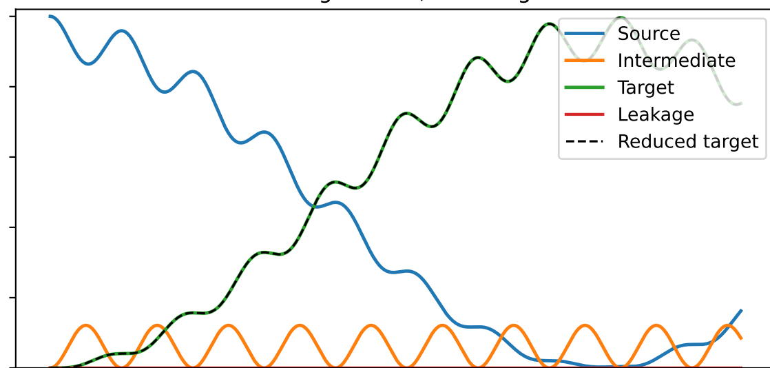
n=1 detuned: g=4 MHz, detuning=20 MHz
