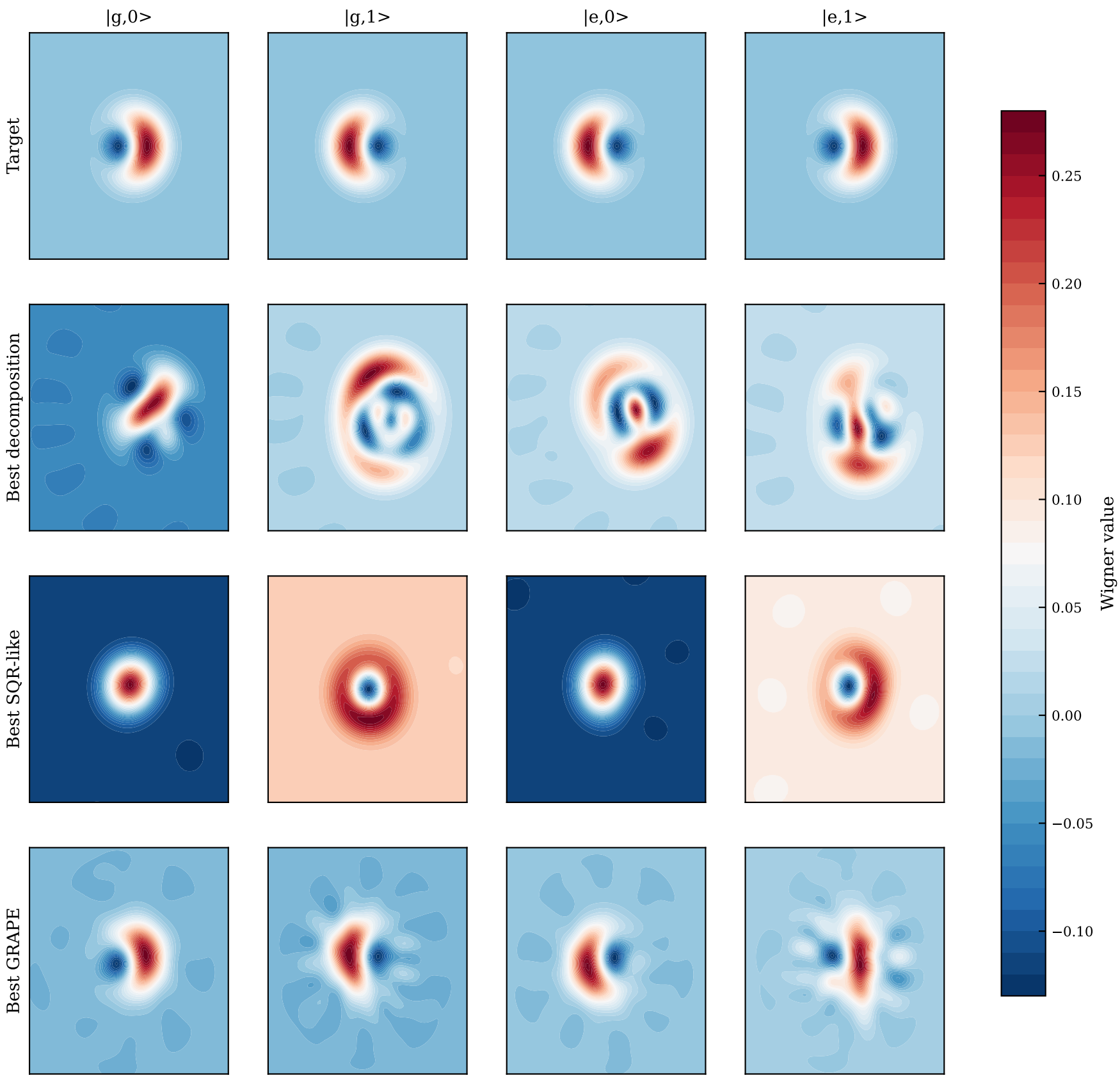
Wigner-function comparisons on logical basis inputs
