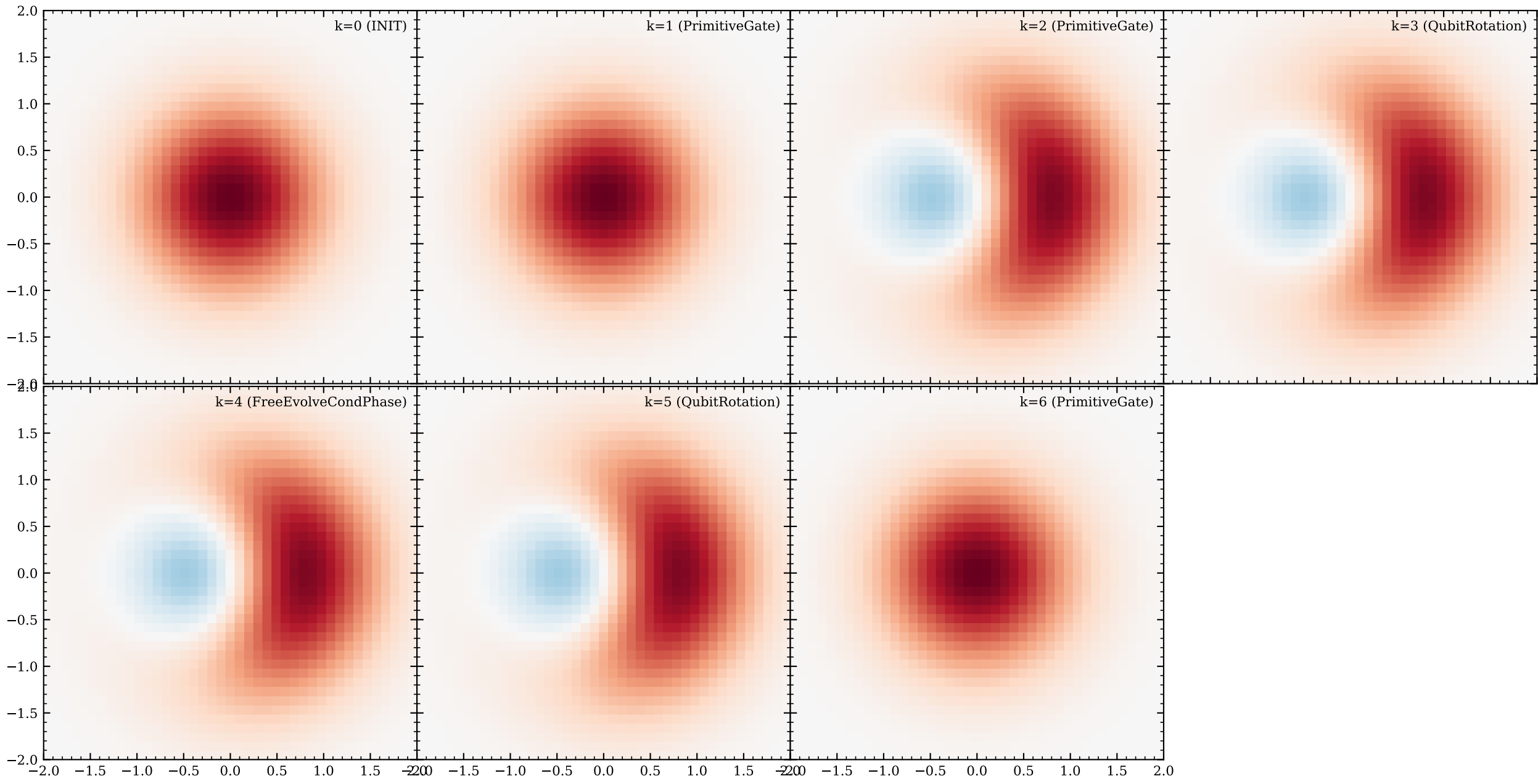
N1_exact_hc_to_exact_hc: cavity Wigner snapshots for g0 (axes: x, p)
