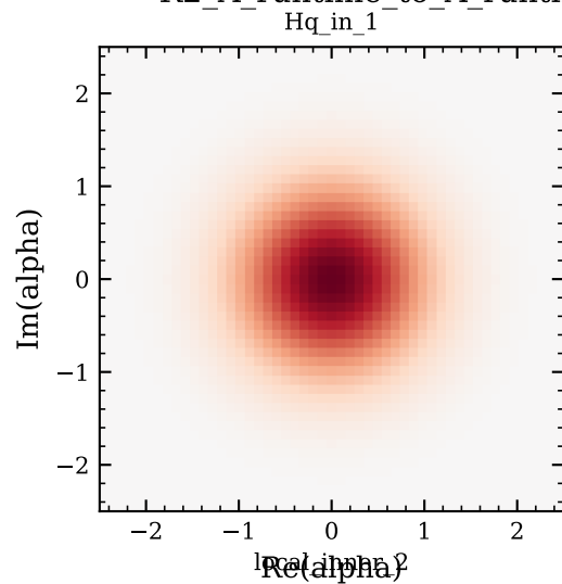
R2_A_runtime_to_A_runtime: Wigner snapshots for g0
