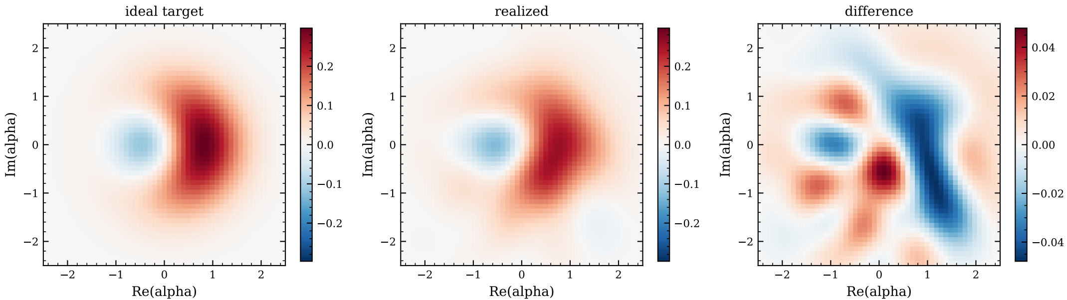
R2_A_runtime_to_A_runtime: final Wigner comparison for g0
