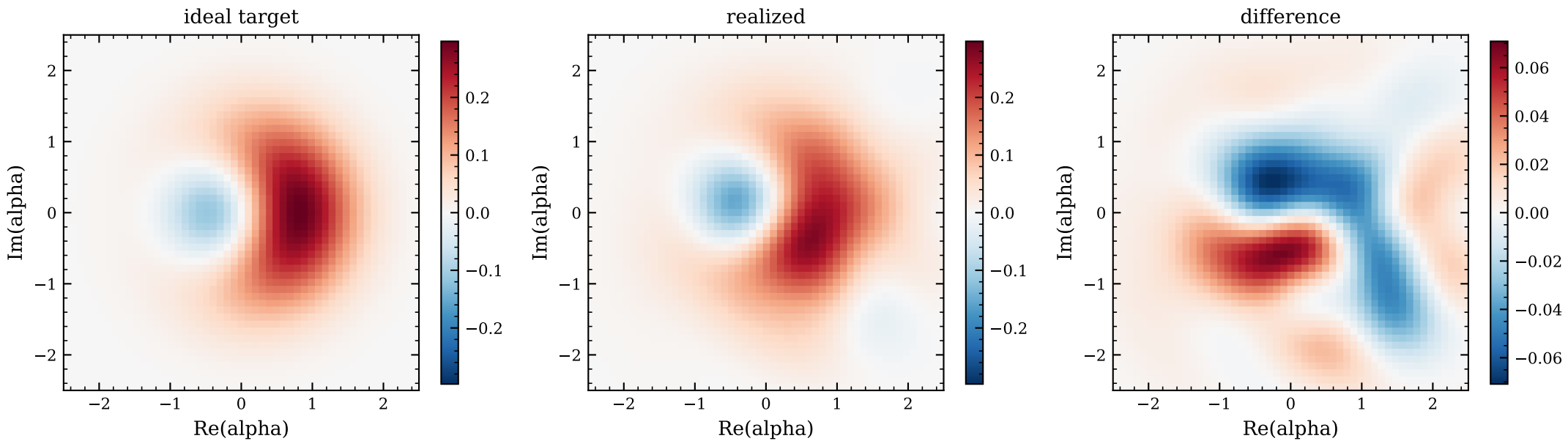
R2_exact_runtime_to_exact_runtime: final Wigner comparison for g0
