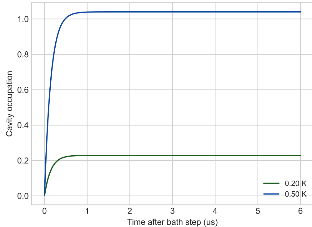
Intrinsic quantum response of cavity
