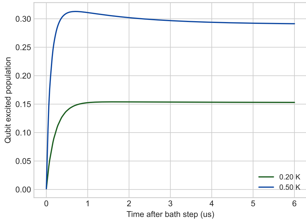
Intrinsic quantum response of qubit thermometer
