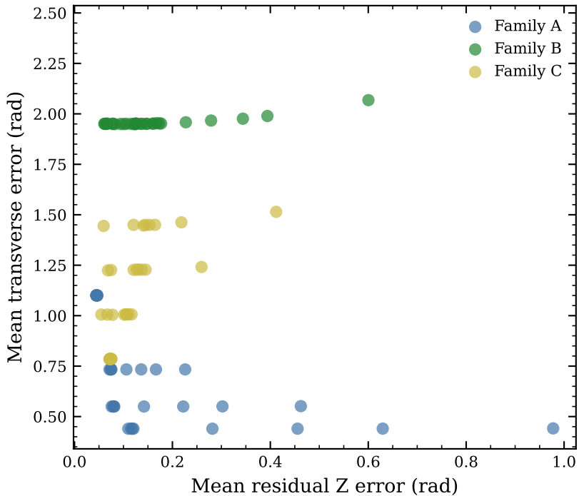
Structured targets
