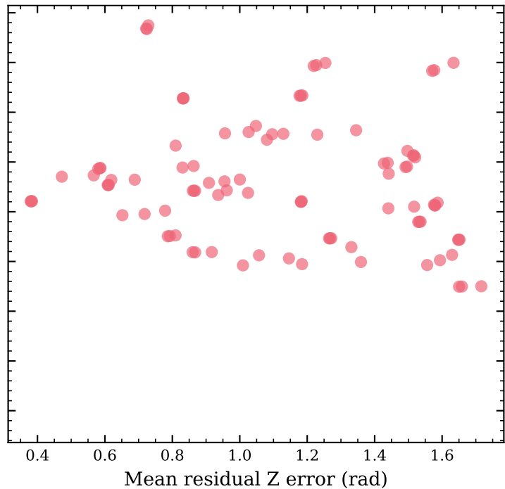
Random targets
