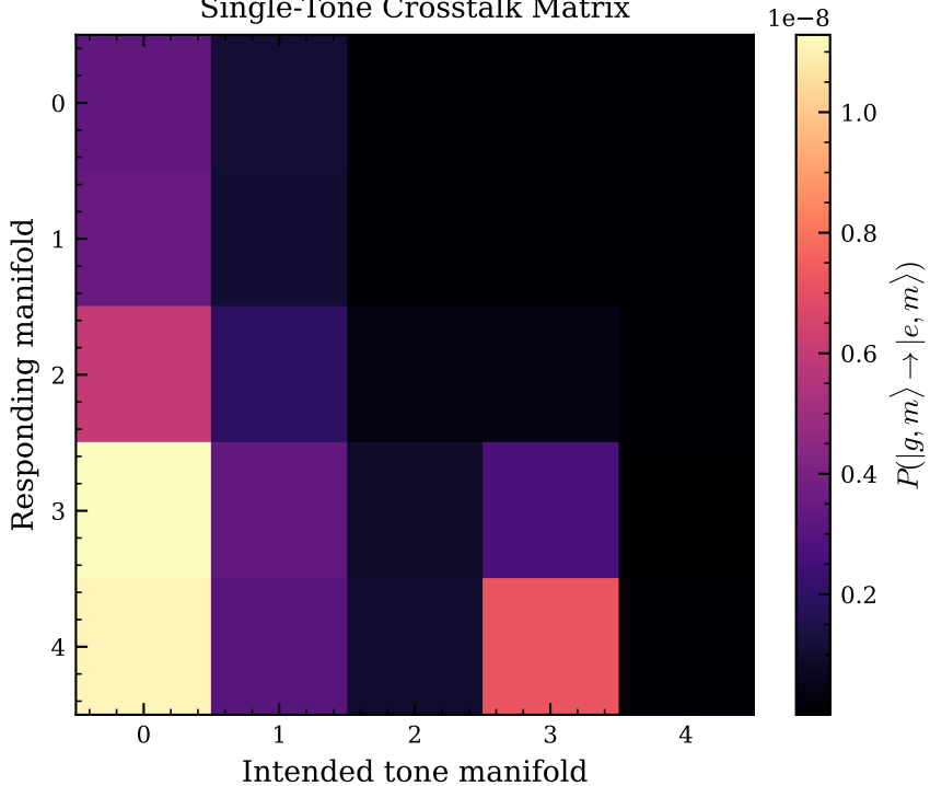
Single-Tone Crosstalk Matrix
