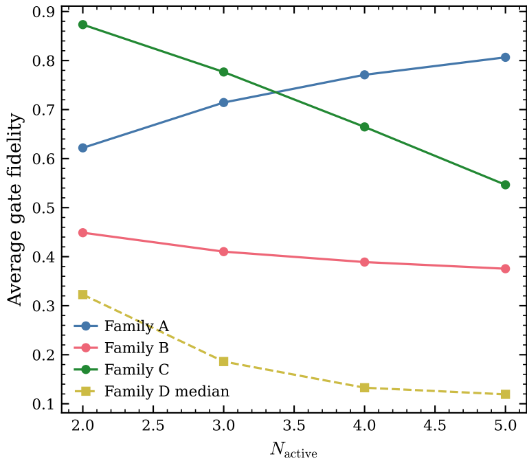
chi only
