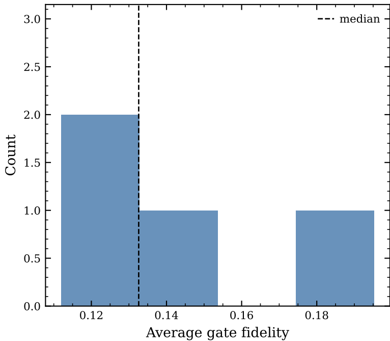
chi only
