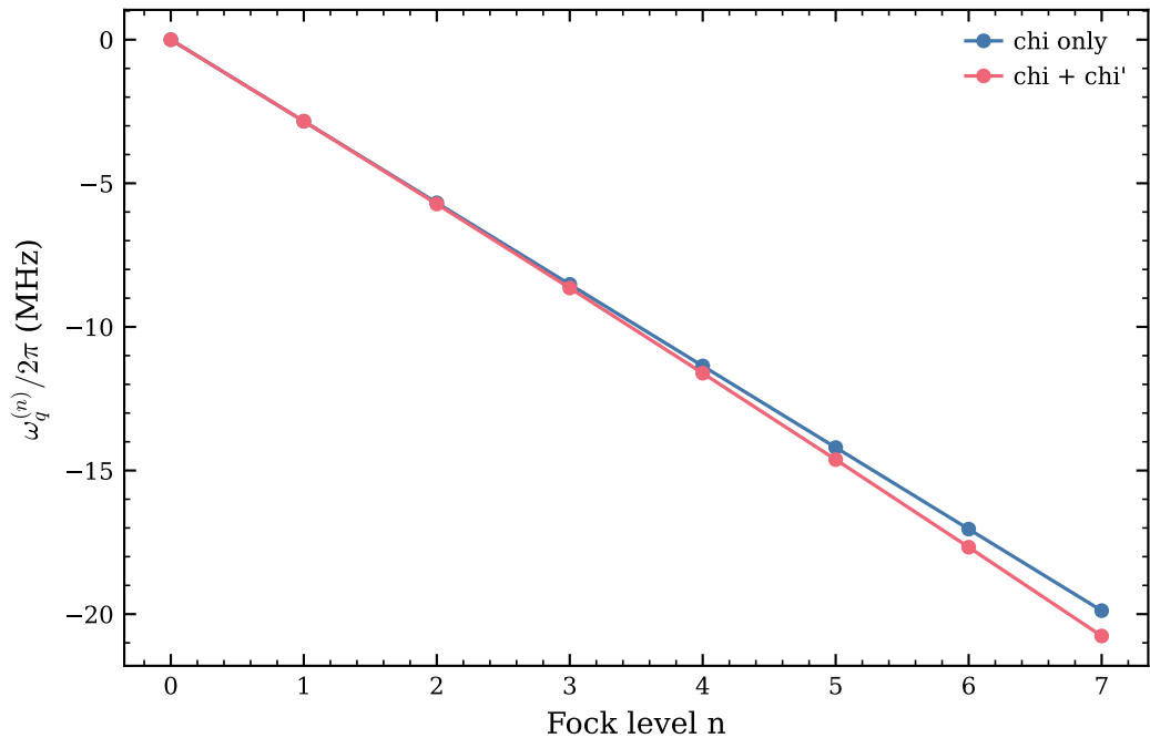
Fock-Conditioned Qubit Transition Frequencies
