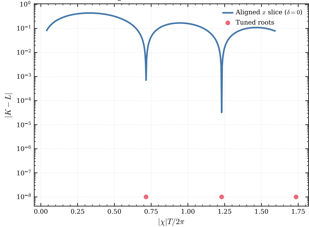
Aligned-x accidental tuned roots
