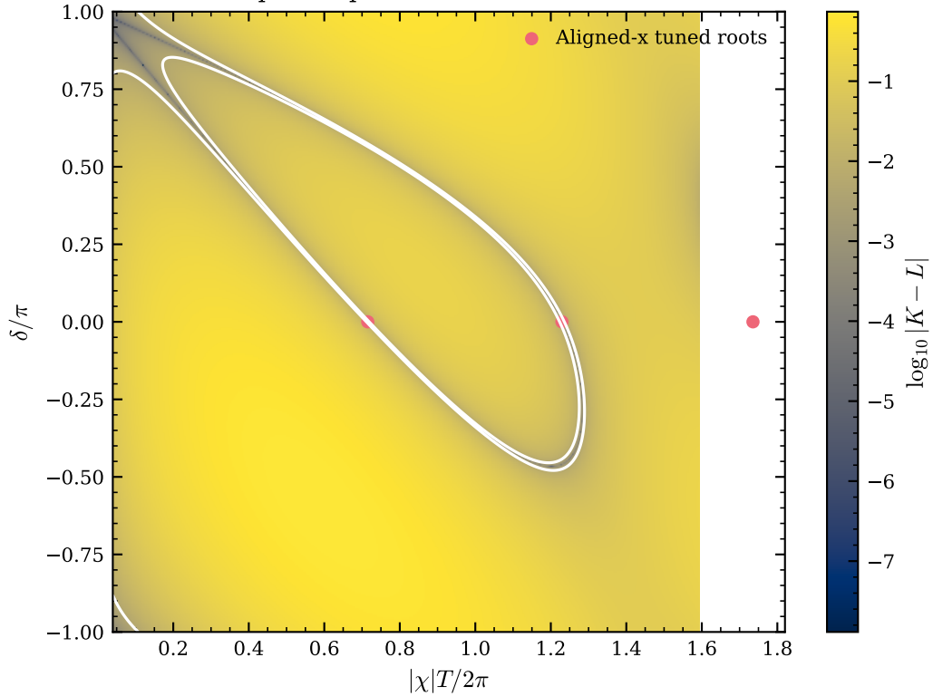
Equal-amplitude tuned-set residual
