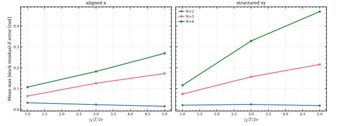
FIG. 2. Mean maximum blockwise residual- Z error versus normalized duration for the strict shared-line model. The residual phase grows with both duration and the size of the addressed manifold window.
