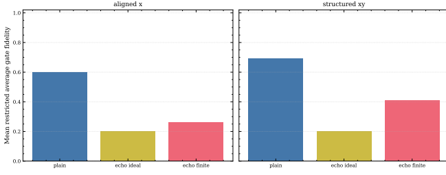
FIG. 4. Mean fidelity comparison for the plain strict multi-tone pulse and the two baseline echoed variants. The ideal instantaneous echo reduces residual- Z accumulation but does not preserve the intended gate, and the simple finite Gaussian echo performs worse because the refocusing pulse is itself manifold dependent.
