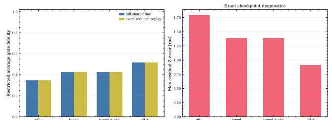
FIG. 7. Exact shared-line checkpoint comparison around the tuned aligned- x locus. The analytically tuned point is special, but not optimal, and no nearby checkpoint realizes an ideal shared-line gate.
