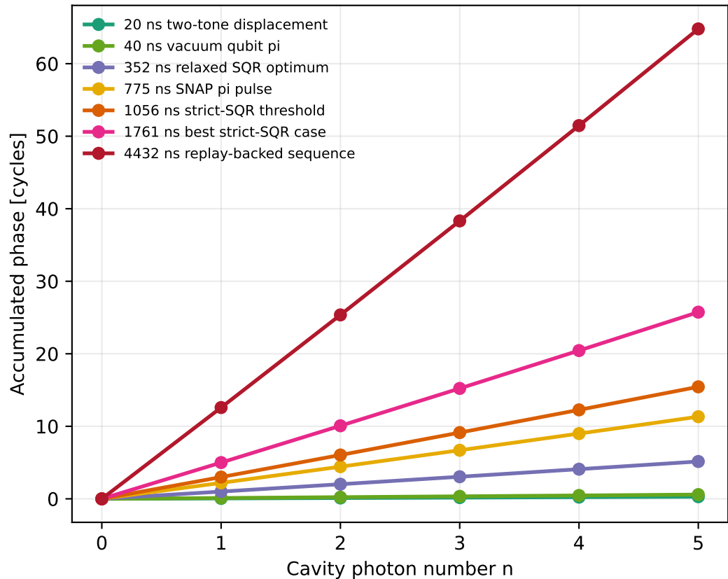
Qubit branch phase from dispersive detuning
