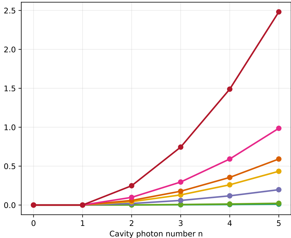
Cavity Kerr phase budget
