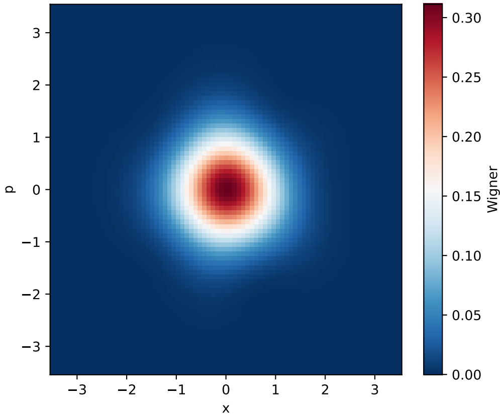
Storage Wigner after ladder cooling
