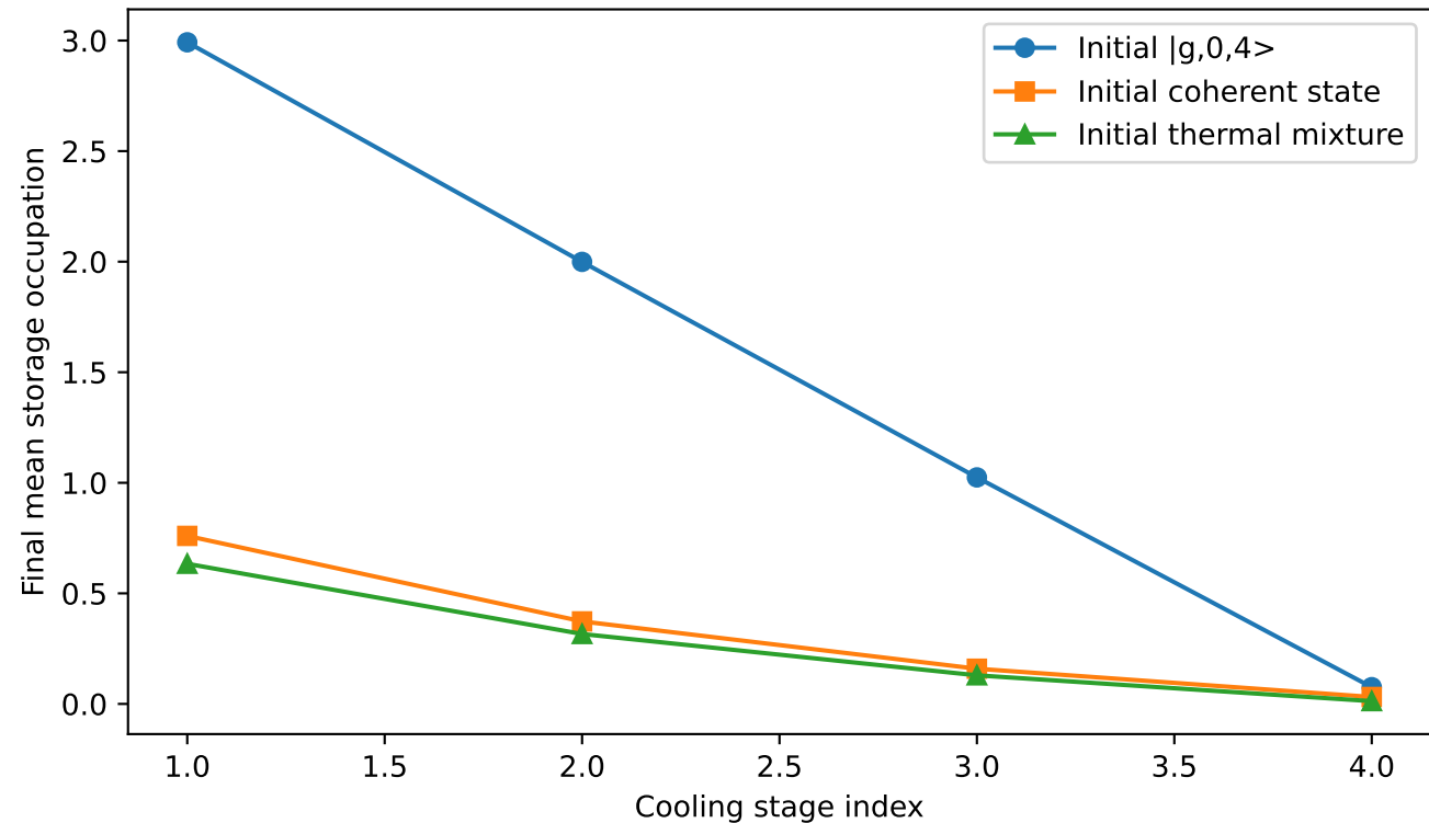
Repeated ladder cooling performance
