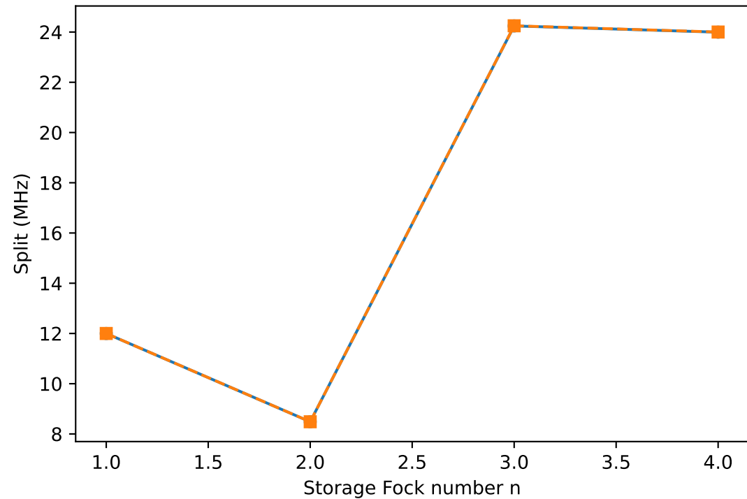
Storage Floquet doublet
