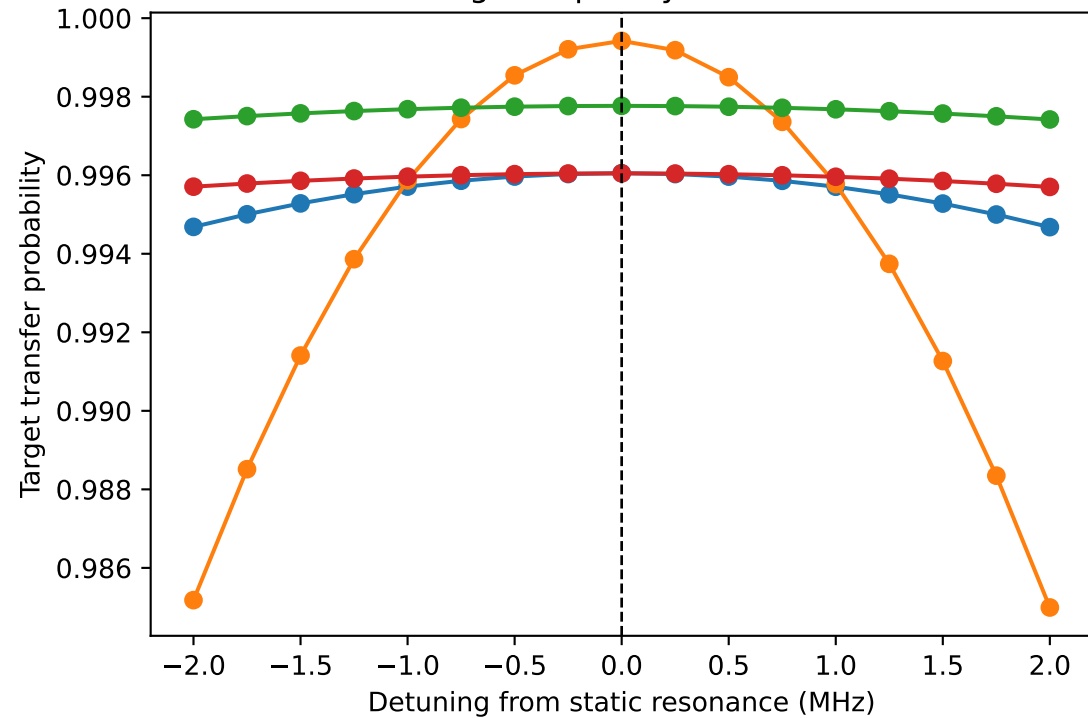
Storage frequency calibration
