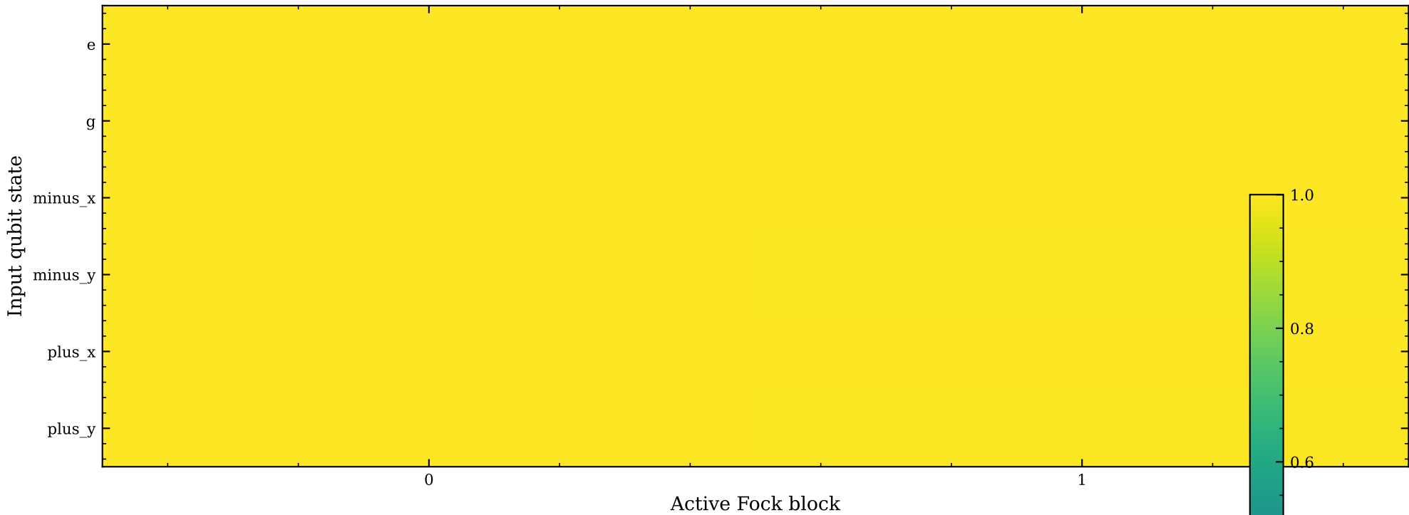
Operator-action validation: segmented_relaxed on random_su2
