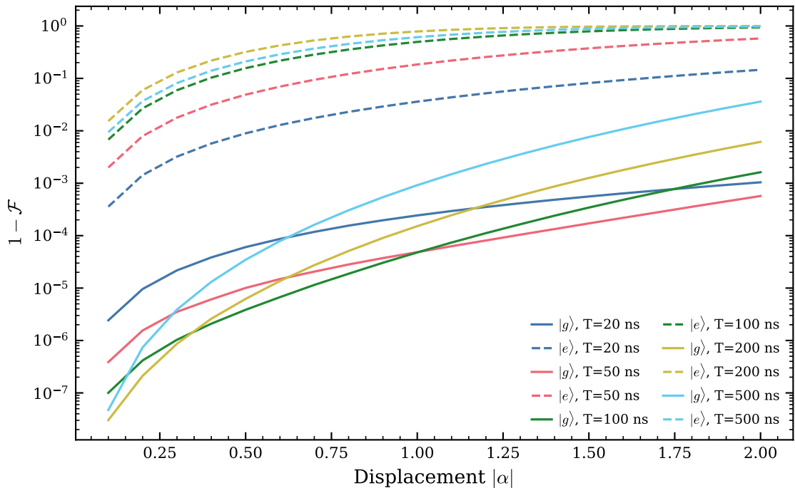
Displacement Infidelity vs. Amplitude
