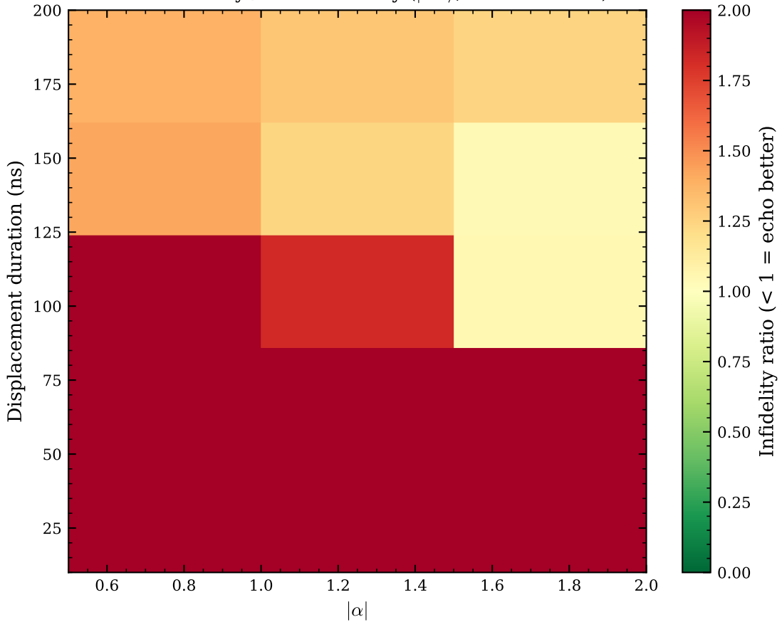
Echo Infidelity / Bare Infidelity ( |+x\rangle , Gauss 20 ns \pi )
