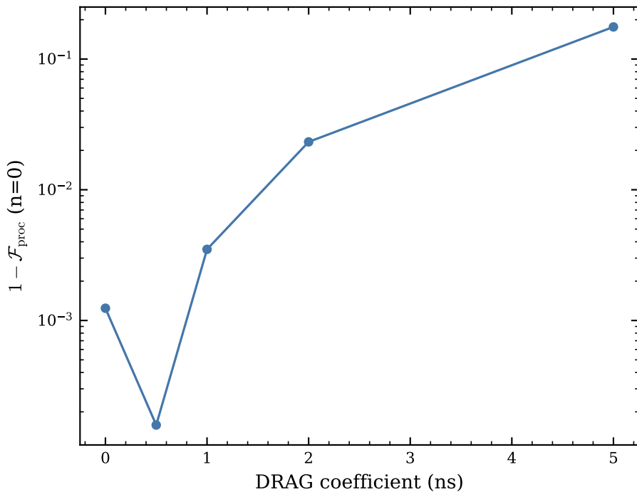
Rotation Infidelity vs. DRAG
