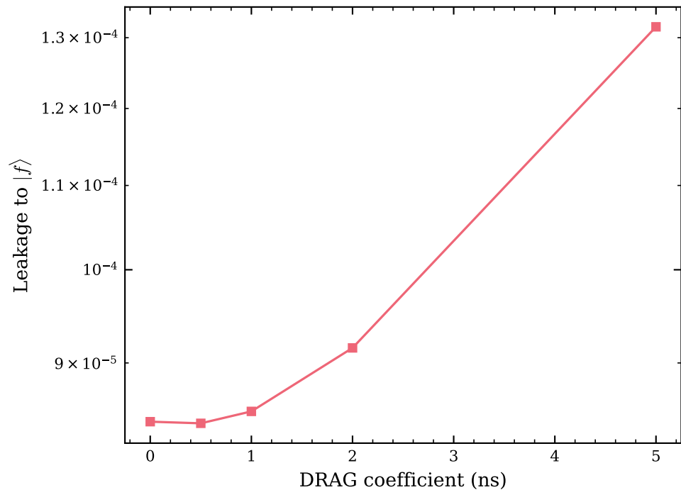
Leakage vs. DRAG
