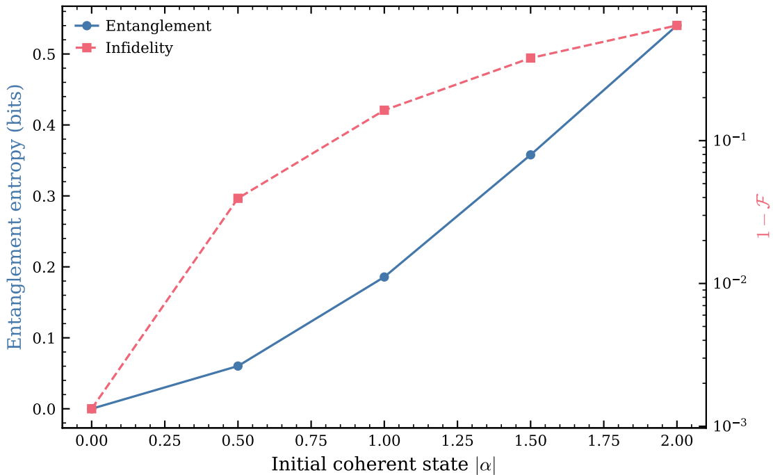
Qubit X_\pi Pulse: Entanglement with Cavity
