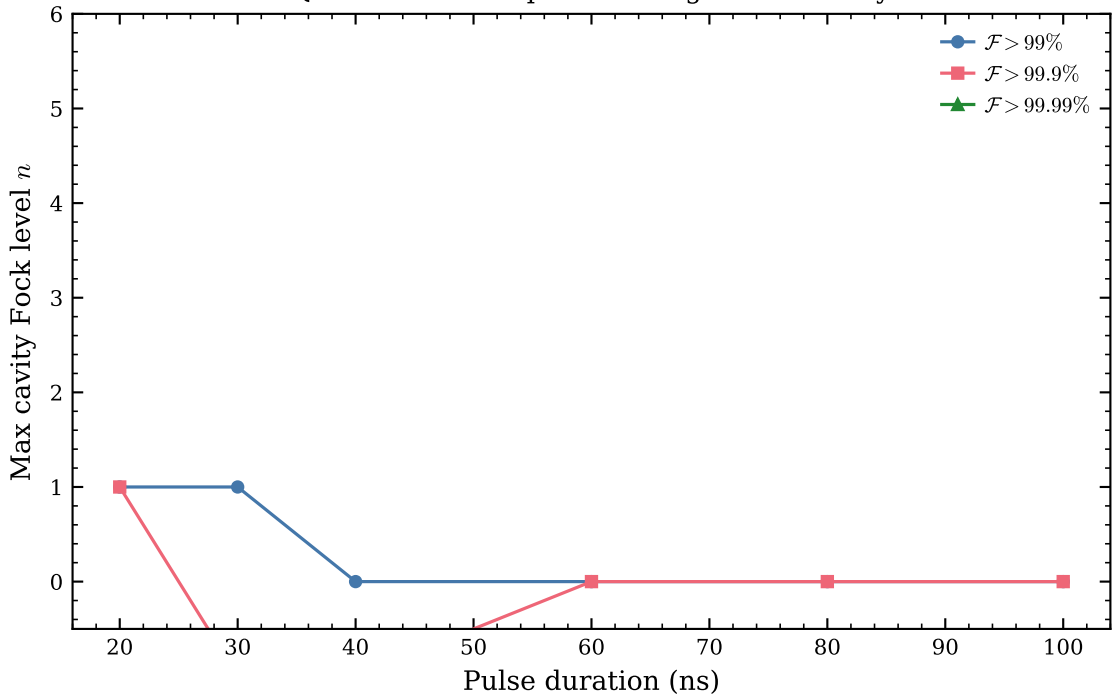
Qubit Rotation: Spectator Regime Boundary
