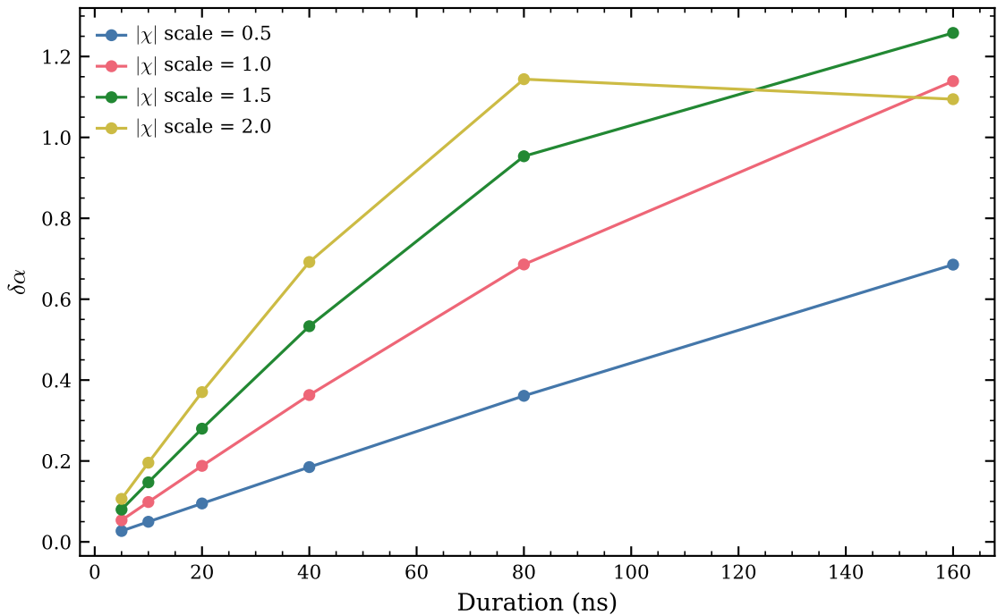
Naive displacement error scaling with |\chi|
