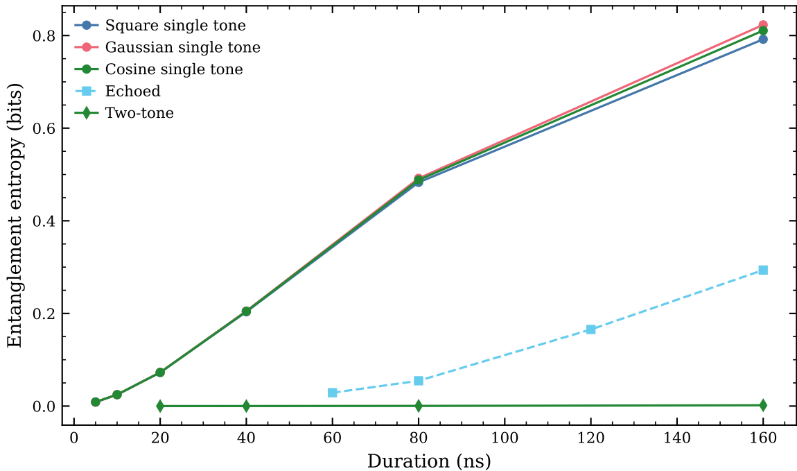
Residual entanglement for |+x\rangle \otimes |0\rangle
