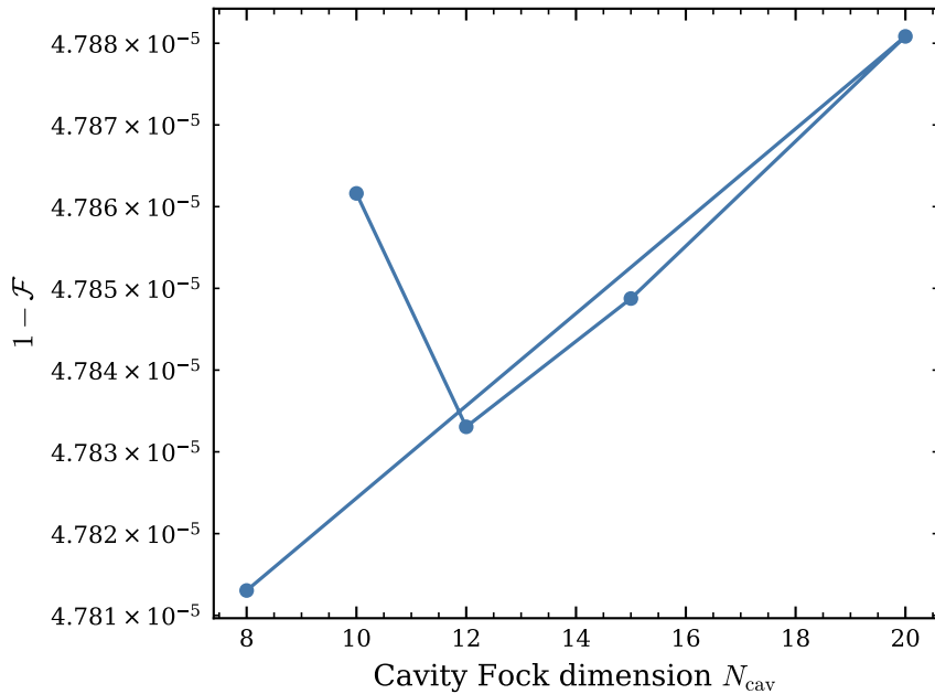
Displacement: N_{\text{cav}} Convergence
