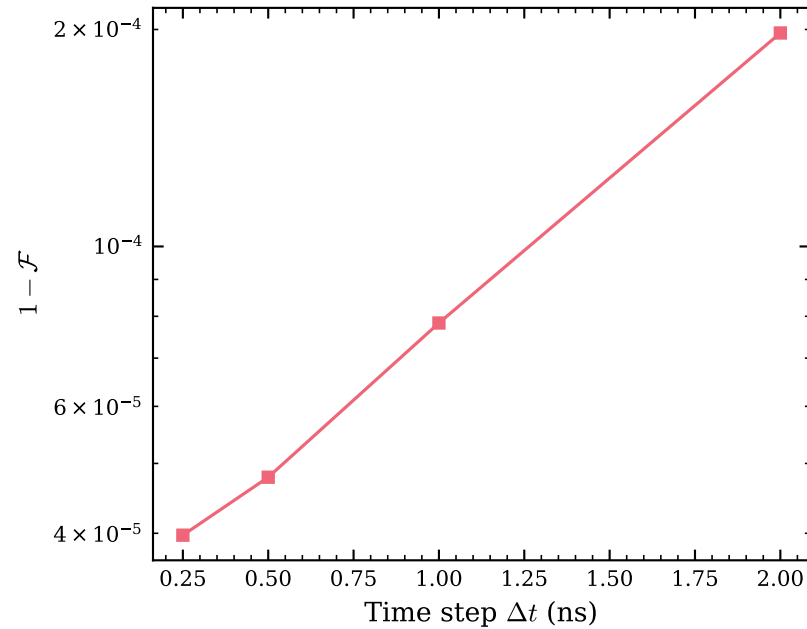
Displacement: \Delta t Convergence
