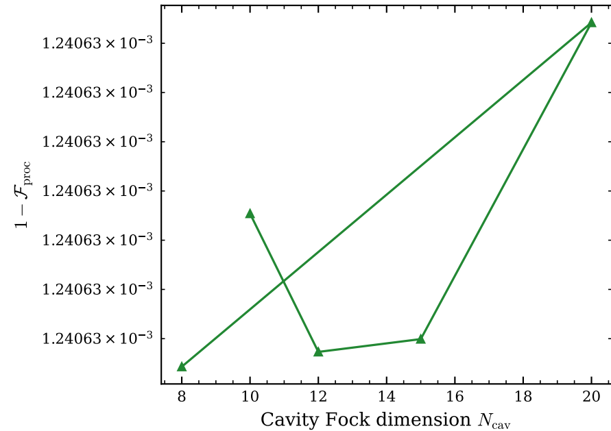
Qubit Rotation: N_{\text{cav}} Convergence
